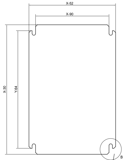
Mounting plate
