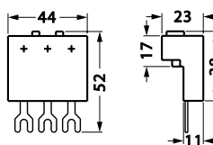
MSP-TA2 three-phase feed-in terminal, type I
