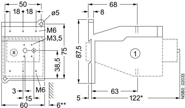
CES-RT3 with CES-AD-RT3 stand-alone adapter
