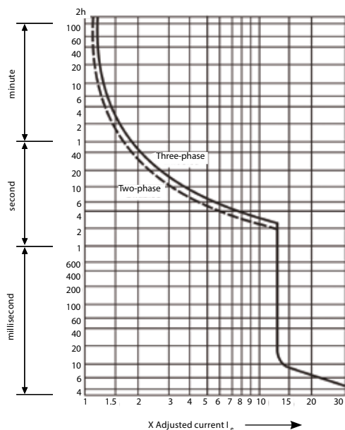
MPE25, MPE80 I-t diagram
