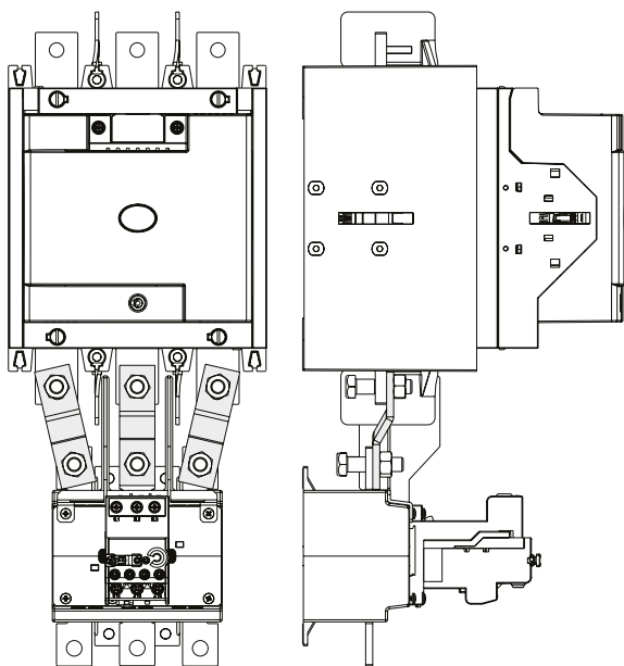
CEM450E/560E + RE317D (200...420A)
