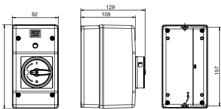
Insulated Enclosure - MPEE55
