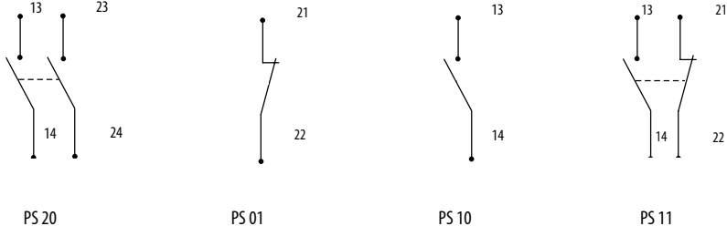
PS designation of contacts
