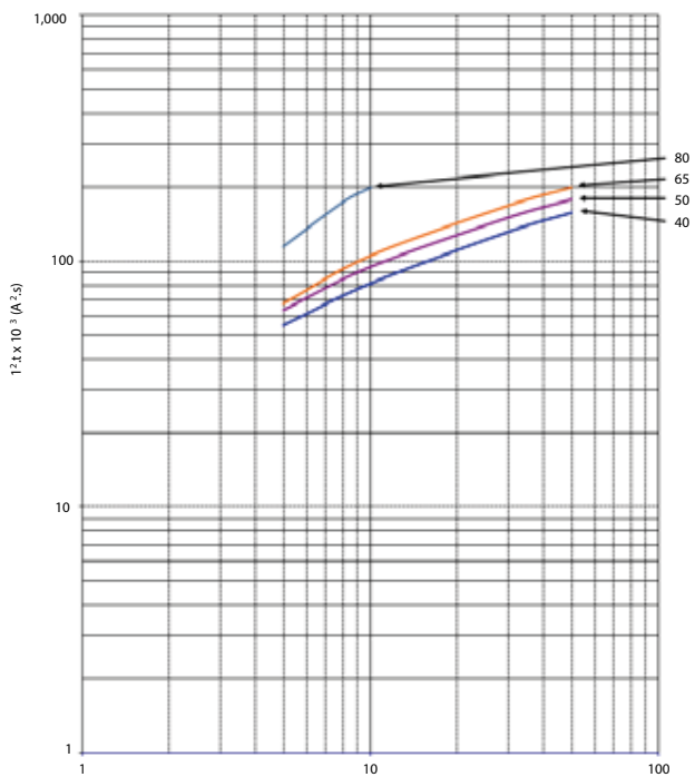
MPE80 Let-through characteristics at 415V
