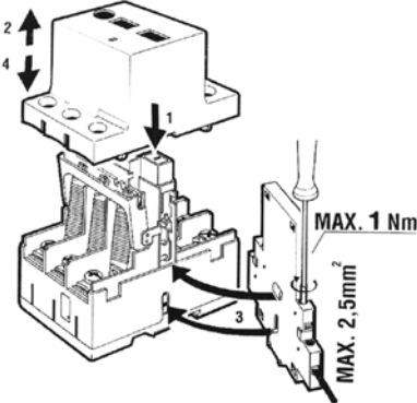
PS mounting
