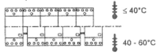
Distance piece
