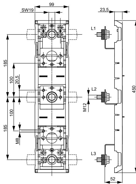
adapter DA 185-100/52
